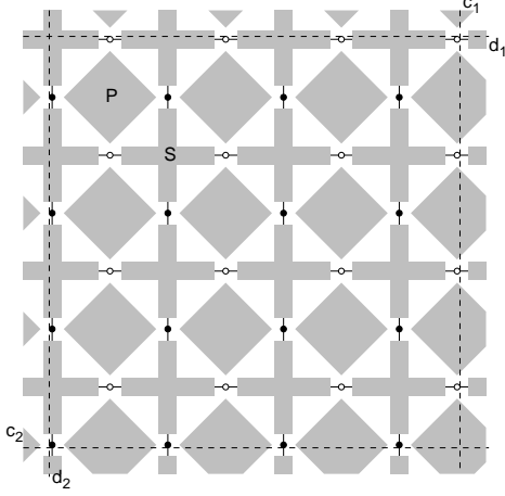
Figure 1: Kitaev's lattice
