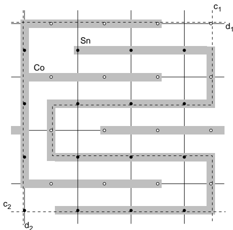
Figure 2: Partitioning Kitaev's lattice
