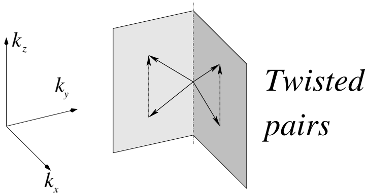
Figure 3: Twisted pairs of momenta for d = 3
