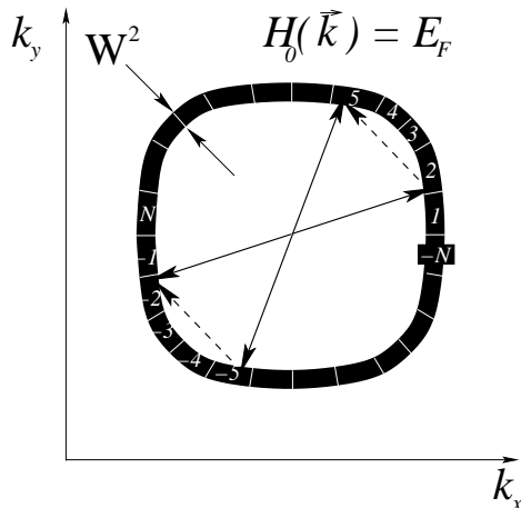
Figure 2: Fermi Surface for the Flip Model
