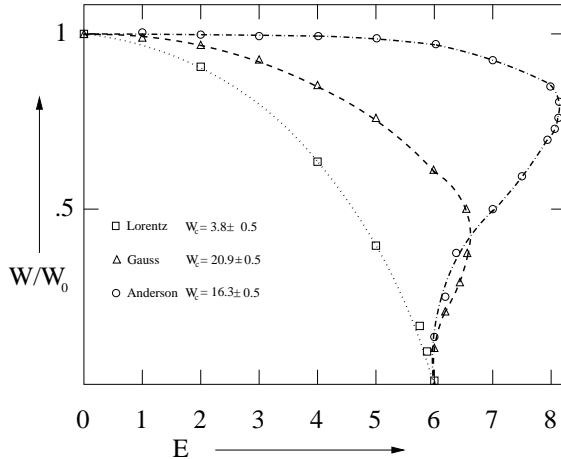
Figure 1: The phase diagram of the 3D Anderson model [29]
