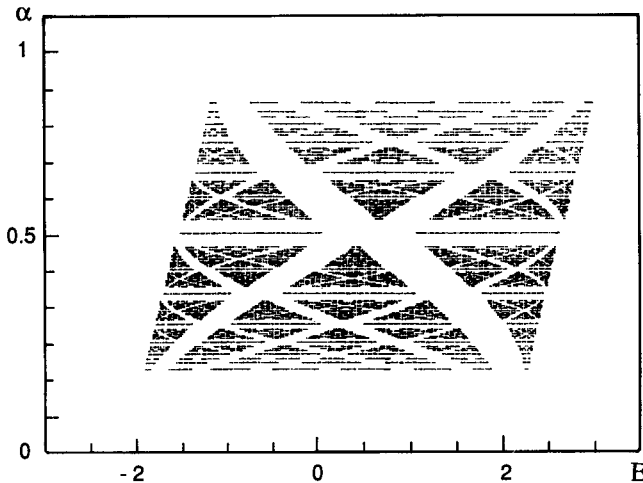
Fig. 1. The energy E has been plotted as a function of \alpha if it is in the spectrum of H(\alpha, x, \lambda) . The coupling constant \lambda is 1 and x=0
